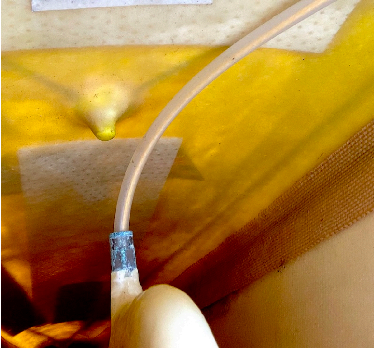
Figure 4.9: Compression fitting in composite boat
