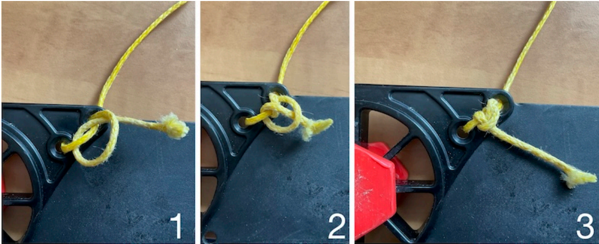
Figure 4.25: Alternative approach to tying off cord on the side of the blade. Whilst there is now no knot above the skeg, the knot does add some bulk to the side of the blade which may catch on the walls of the skeg box.
