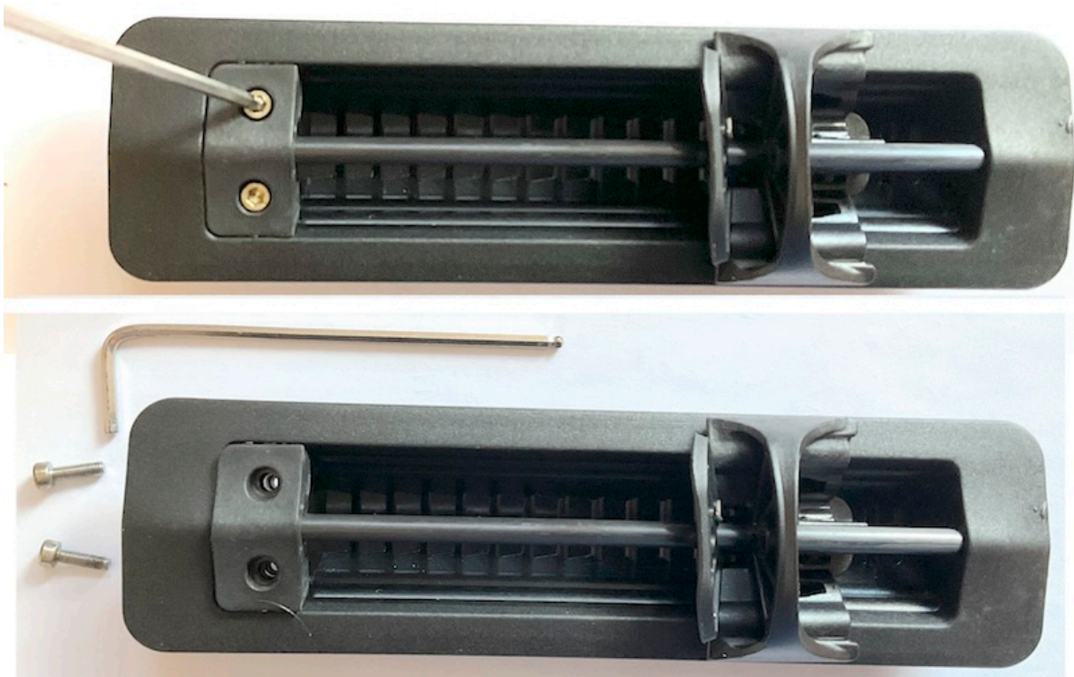
Figure 3.1: 1.Undo both of the screws with the 2.5 mm Allen key and remove them.
