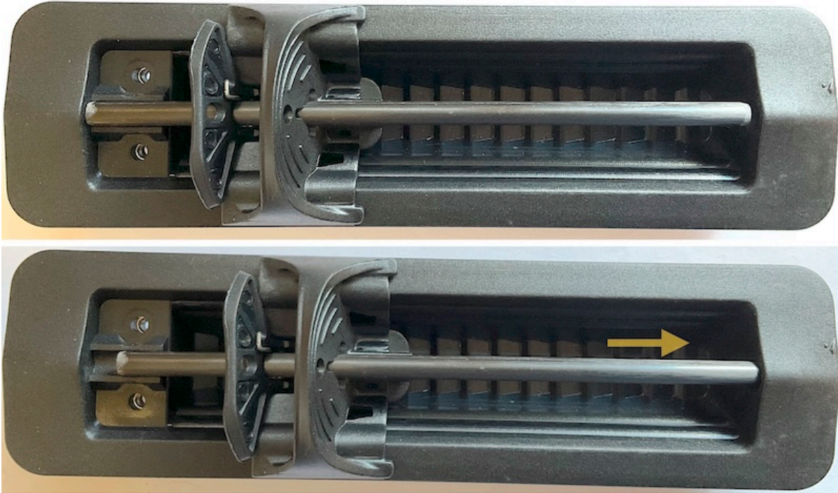
Figure 3.7: The rod and slider are placed in the ratchet box. Check that the slider is assembled in the correct orientation, as shown - the hole for the cord should be towards the stern of the boat and the lever towards the bow. The rod is then slid backward into the hole in the ratchet box.
