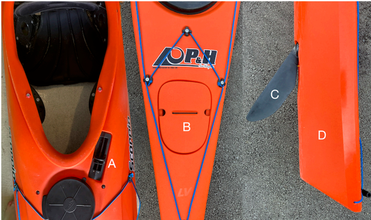
Figure 1.4: Boat with skudder-type skeg, showing new controller position (A), actuator cover (B) and new blade (C) that deploys near the stern of the boat (D).
