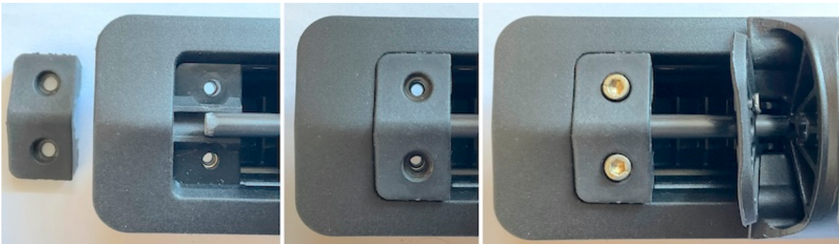
Figure 3.8: Verify that the rod is slid back, such that the retainer drops into place easily. Place the retainer into place, checking that its orientation is correct - the rounded corners go towards the bow to fit with the rounded corners of the ratchet box. Replace the screws.
