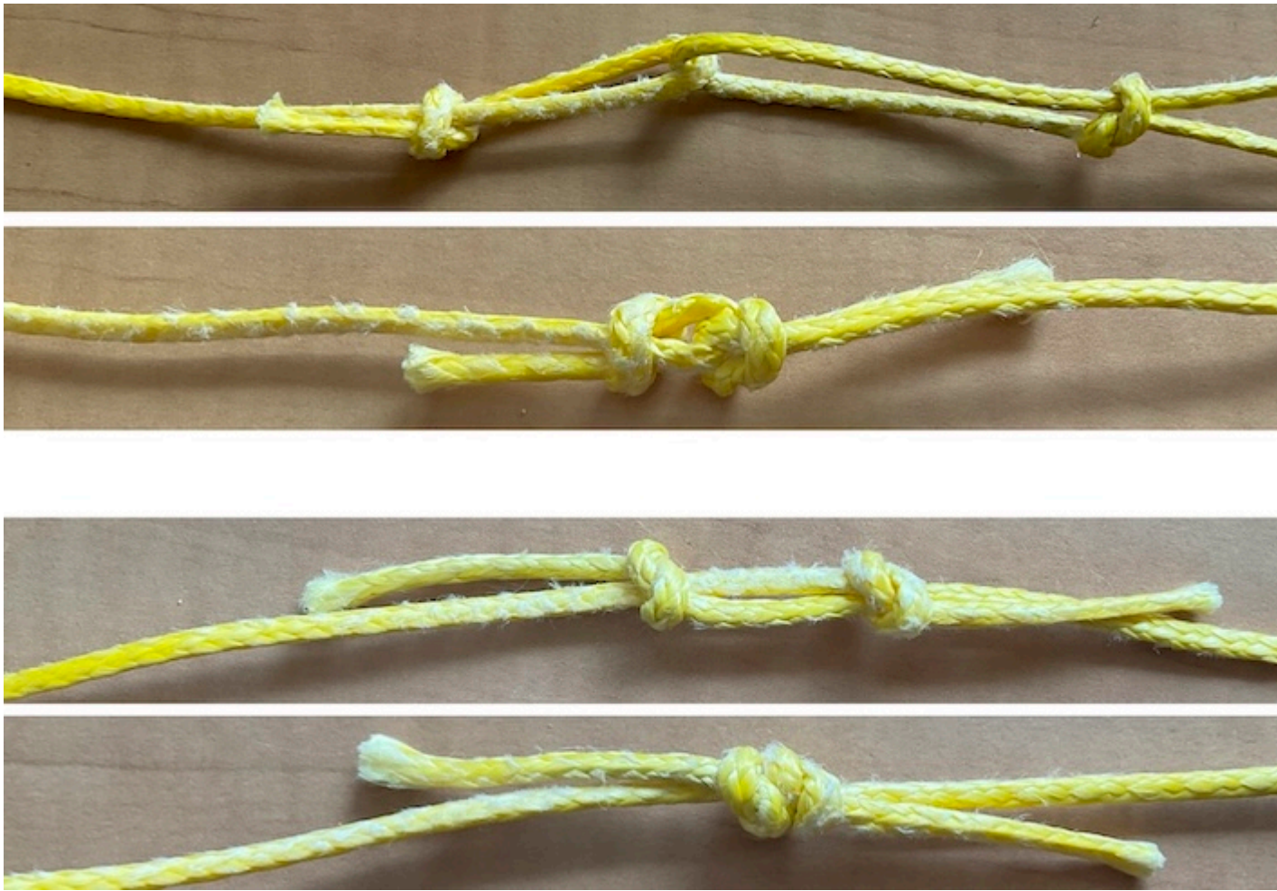
Figure 4.19: 2 possible knots to tie the cords together. The top two images show knots forming interlocked loops. The bottom shows a fisherman's bend.
