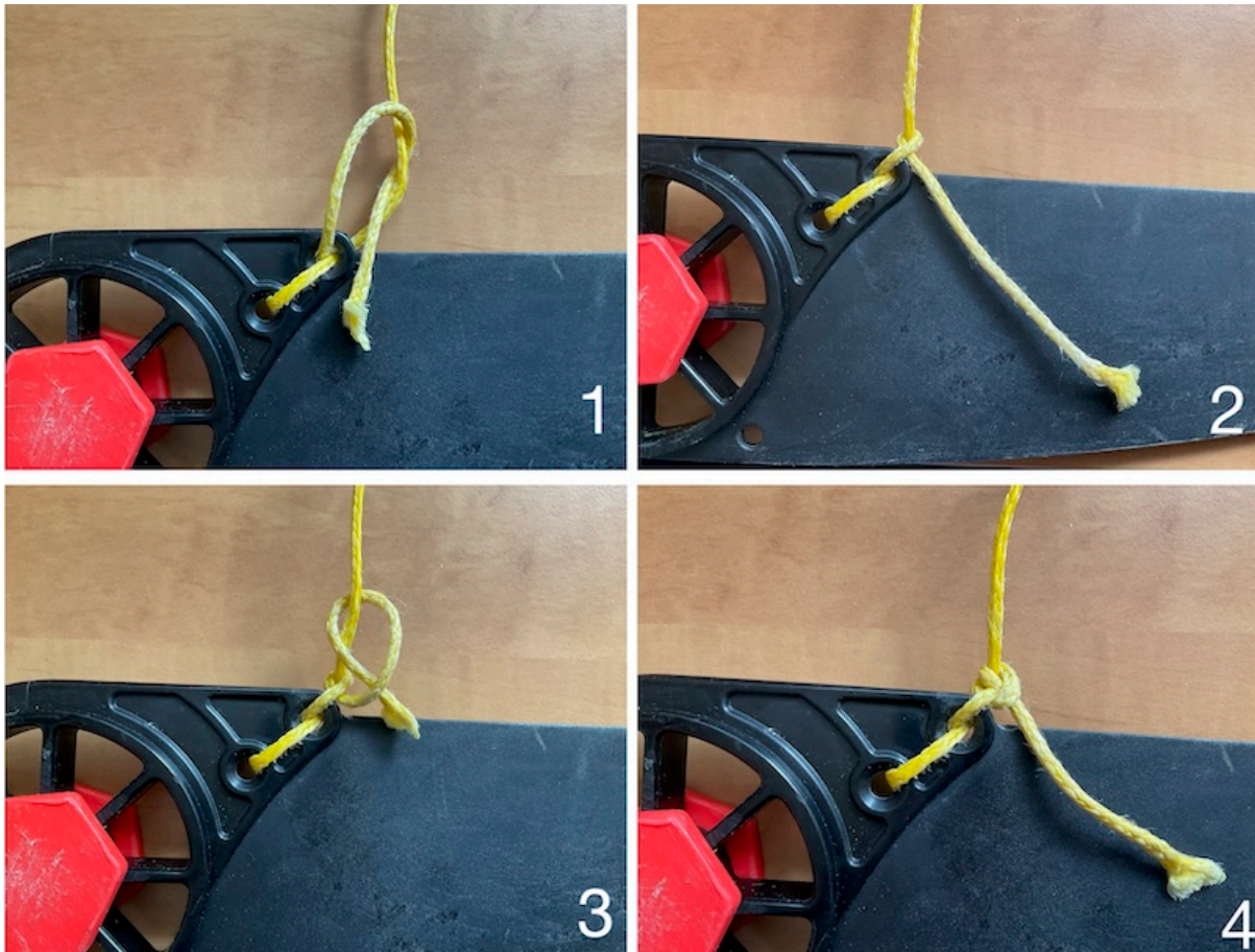
Figure 4.24: One approach to knotting the cord onto the blade with half hitches above the blade. This tends to work well, but the knot might hit the end of the tube preventing the blade fully retracting. In practice, this doesn't seem to be a problem.
