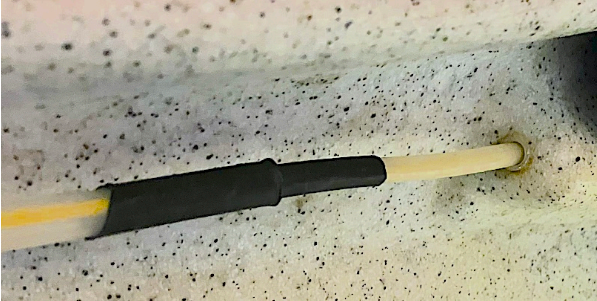
Figure 4.6: Compression fitting termination in boat with 8mm tube. The 8mm tube is connected to a short length of 6mm tube with some black heat shrink. The 6mm tube goes into a push fitting bonded to the hole in the boat at the back of the slider box.
