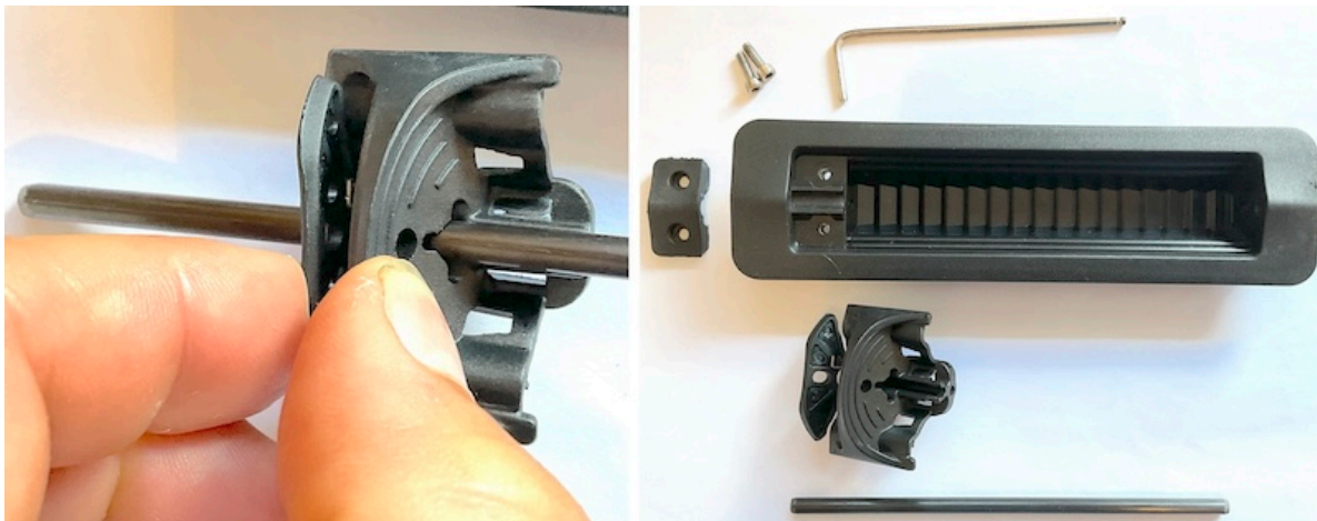
Figure 3.3: 3.Once the bar is removed, squeeze the lever to the button on the slider and slide it off the bar.
