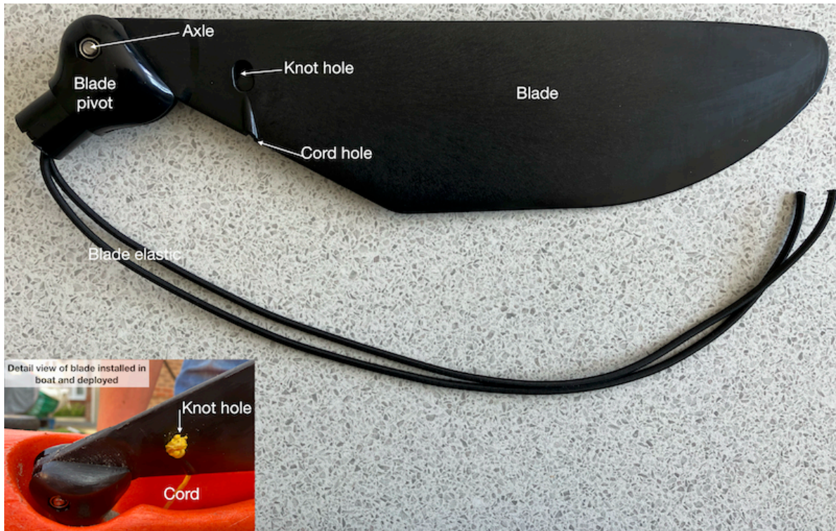
Figure 5.7: Skudder-type blade assembly removed from boat
