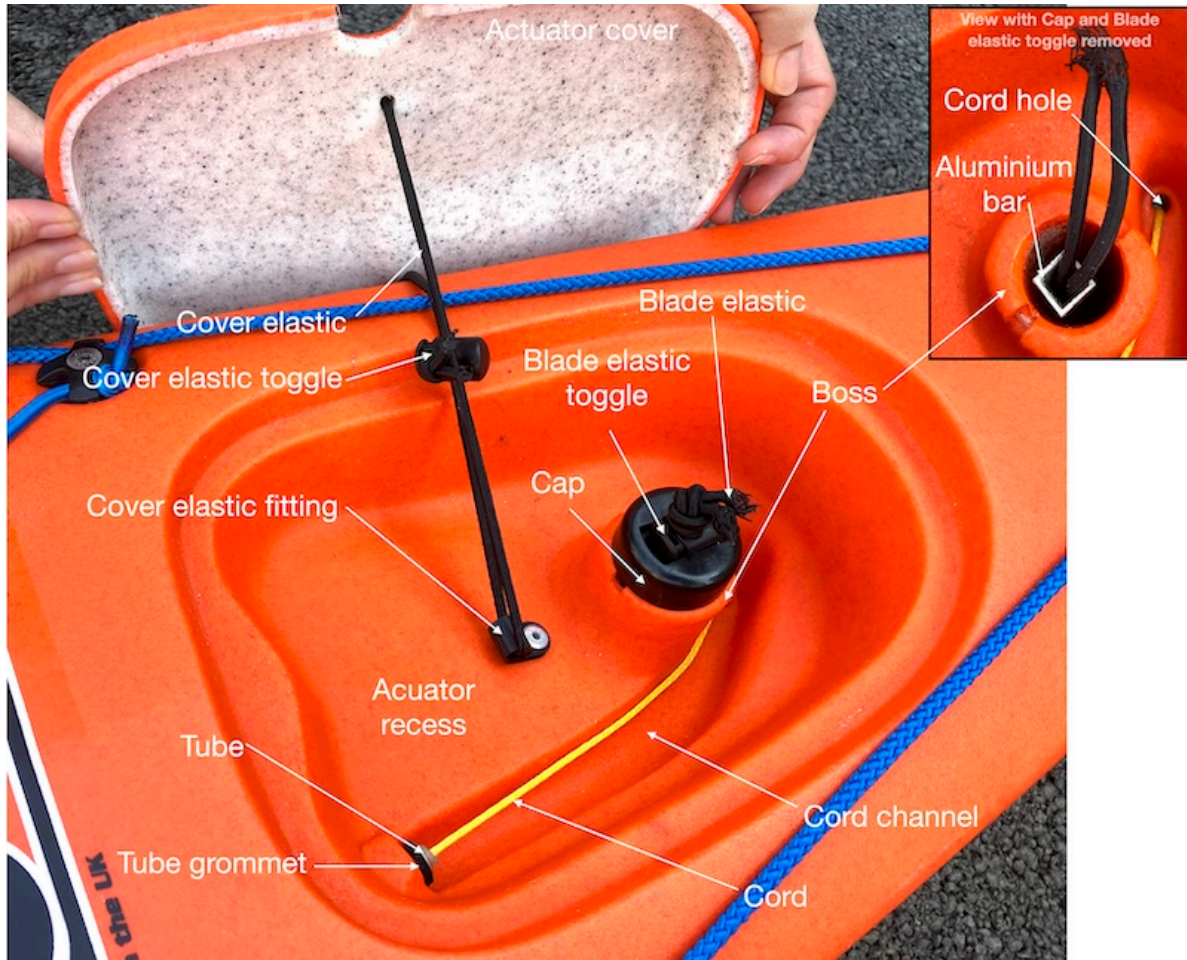
Figure 5.6: The Actuator Recess with cover pulled aside
