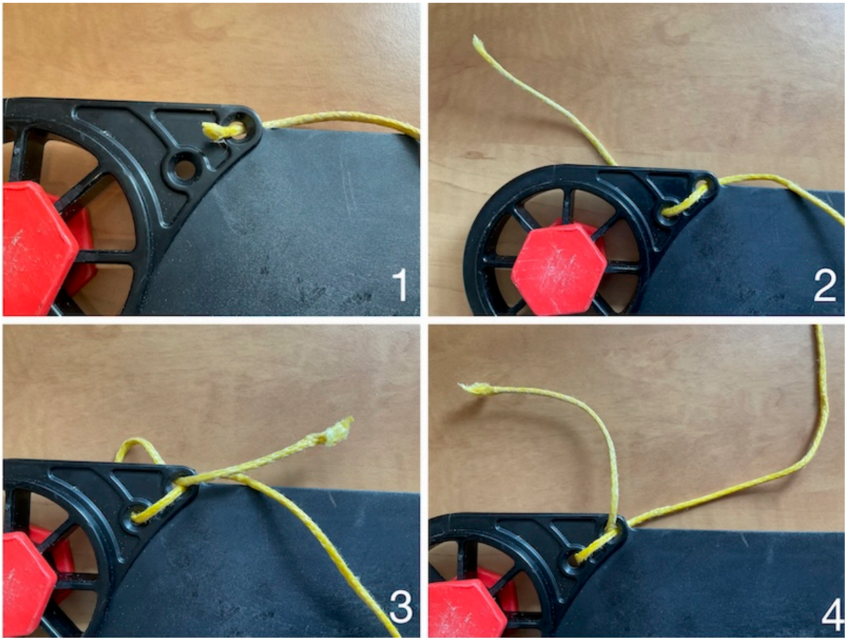
Figure 4.23: Threading the cord onto the blade
