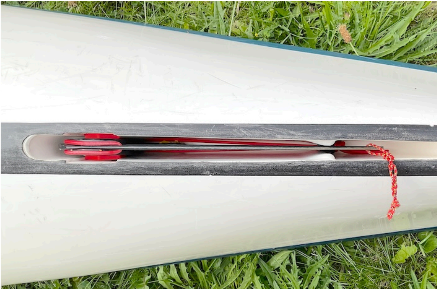
Figure 5.1: Looking into the skeg box from the bottom of the boat. Note the red elastic running around the grooves in the blade and to the ferrule in the back of the skeg box. The red axle component is also visible.
